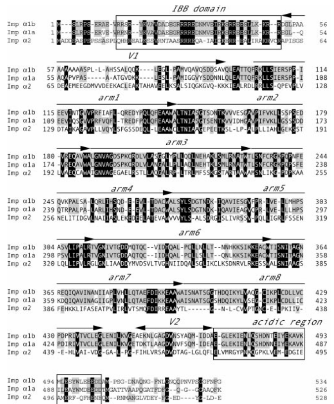
Fig. 1. Multiple sequence alignment of rice importin \alpha s. Protein sequences were aligned using GENETYX genetic information processing software (Software Development Co., LTD, Tokyo, Japan). Identical amino acid residues across either all three or two of the clones are indicated by black and gray boxes, respectively. IBB domain, arm repeats ( arm ), variable region (V), and two variable regions flanking the arm repeats region (Fig. 1).
