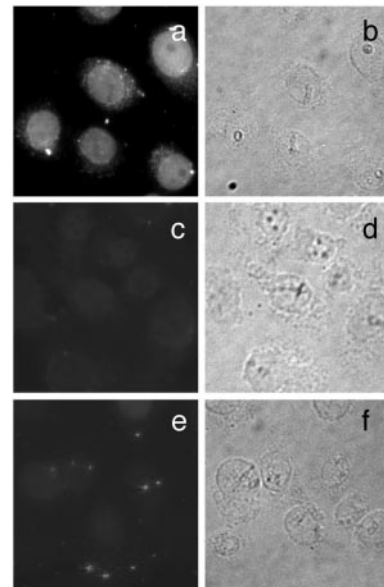
FIG. 3. The effect of rice importin \alpha 1b on the nuclear binding and import of GST-NLS-GFP assayed in vitro using digitonin-permeabilized HeLa cells. Part A, for nuclear binding, a 10- \mu l assay sample was incubated on ice for 20 min. GST-NLS-GFP was 0.2 \mu g; rice importin \beta 1 was 6 pmol; rice importin \alpha 1b was 6 pmol. Part B: for nuclear import, a 10- \mu l assay sample was incubated at 25 ^{\circ} C for 20 min in the presence of mouse Ran-GDP (42 pmol), 1 mM ATP, 20 units/ml creatine phosphokinase, 5 mM creatine phosphate, and 1 mM GTP. GST-NLS-GFP was 0.2 \mu g; rice importin \beta 1 was 3 pmol; and rice importin \alpha 1b was 12 pmol. In both parts A and B: a and b, T-GFP + importin \beta 1 + importin \alpha 1b; c and d, T-GFP + importin \beta 1; and e and f, Tm-GFP + importin \beta 1 + importin \alpha 1b. After incubation, cells were fixed with 3.7% formaldehyde in TF. Panels a, c, and e, fluorescence images; panels b, d, and f, Nomarski images.
