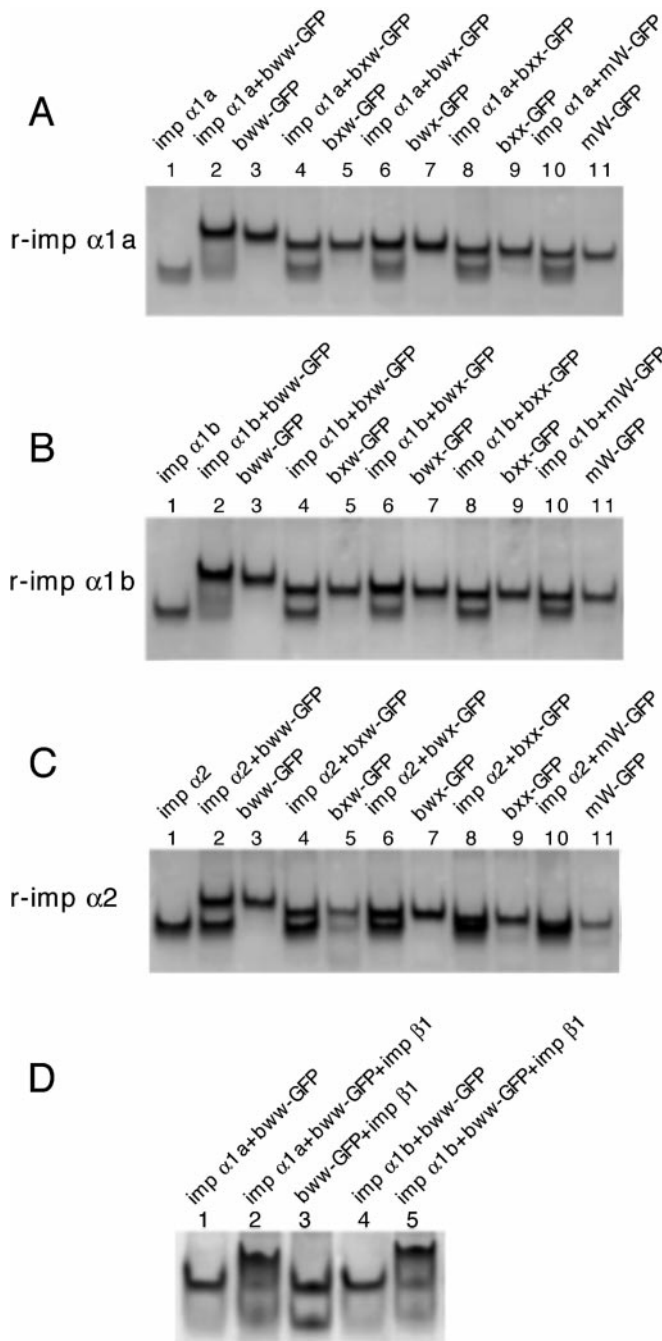
FIG. 6. In vitro interactions between rice importin \alpha s and COP1 NLSs. Native gel electrophoresis was carried out as described in the legend to Fig. 2.
