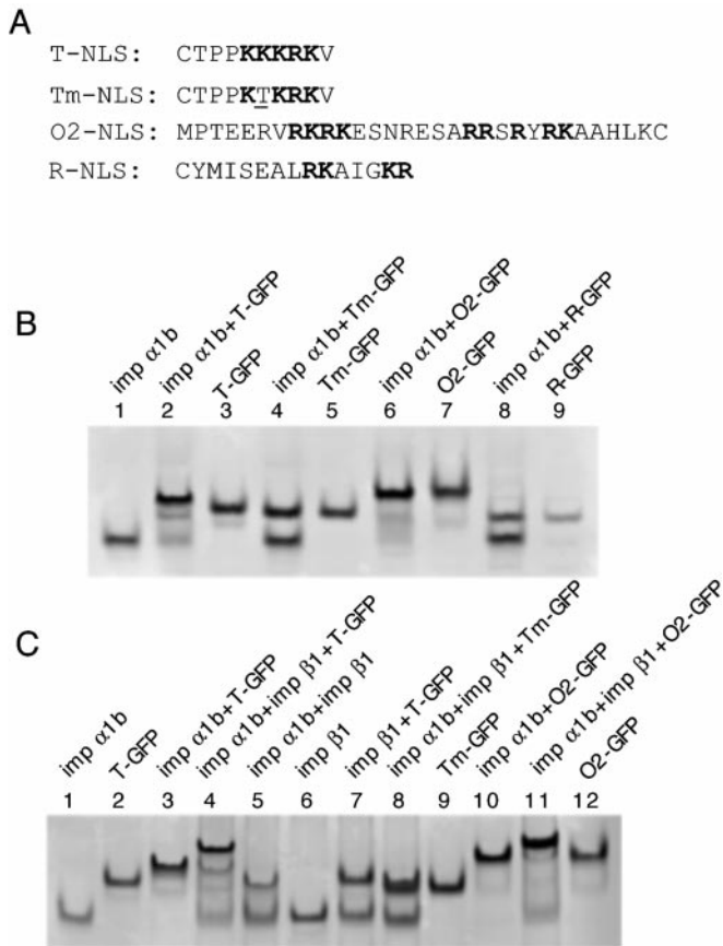
FIG. 2. In vitro protein binding analyses. A, amino acid sequences of SV40 large T-antigen NLS ( T-NLS ), mutant T-NLS ( Tm-NLS ), maize transcription factor opaque 2 NLS ( O2-NLS ), and maize transcription factor R NLS ( R-NLS ) are shown in a single-letter code. Basic amino acid clusters are indicated in bold face and amino acid replacement in Tm-NLS is underlined . These NLSs were inserted between GST and GFP to generate recombinant GST-NLS-GFP fusion proteins designated T-, Tm-, O2-, and R-GFP, respectively. B and C, in vitro protein binding assays were analyzed by native gel electrophoresis. 20 pmol of each protein was mixed in 15 \mu l of transport buffer (TB) (20 mM Hepes, pH 7.3, 110 mM potassium acetate, 2 mM magnesium acetate, 5 mM sodium acetate, 0.5 mM EGTA, 2 mM dithiothreitol, 1 \mu g/ml each of aprotinin, leupeptin, and pepstatin A) supplemented with 250 mM sucrose and incubated for 1 h at room temperature. 7.5% polyacrylamide gels were run in the presence of 1 mM dithiothreitol and 1 mM EGTA in both the gels and the running buffer and stained with Coomassie Blue.
