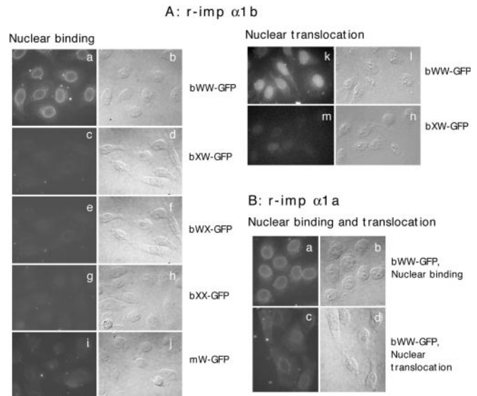
FIG. 7. Preferential nuclear translocation of bWW-GFP by rice importin \alpha 1b . Nuclear binding and import assays were carried out as described in the legend to Fig. 3.
