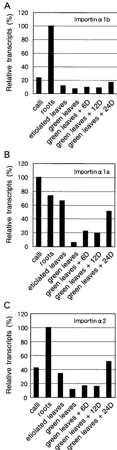
FIG. 4. Transcript analyses of rice importin \alpha s. Total RNA samples were prepared from tissues of either dark-(etiolated leaves) or light-grown (green leaves and roots) rice plants (14-days-old). For dark adaptation, the light-grown plants were further grown in complete darkness for the indicated hours (6, 12, and 24 days, respectively). In each panel, the highest transcript levels were regarded as 100% of relative expression.
